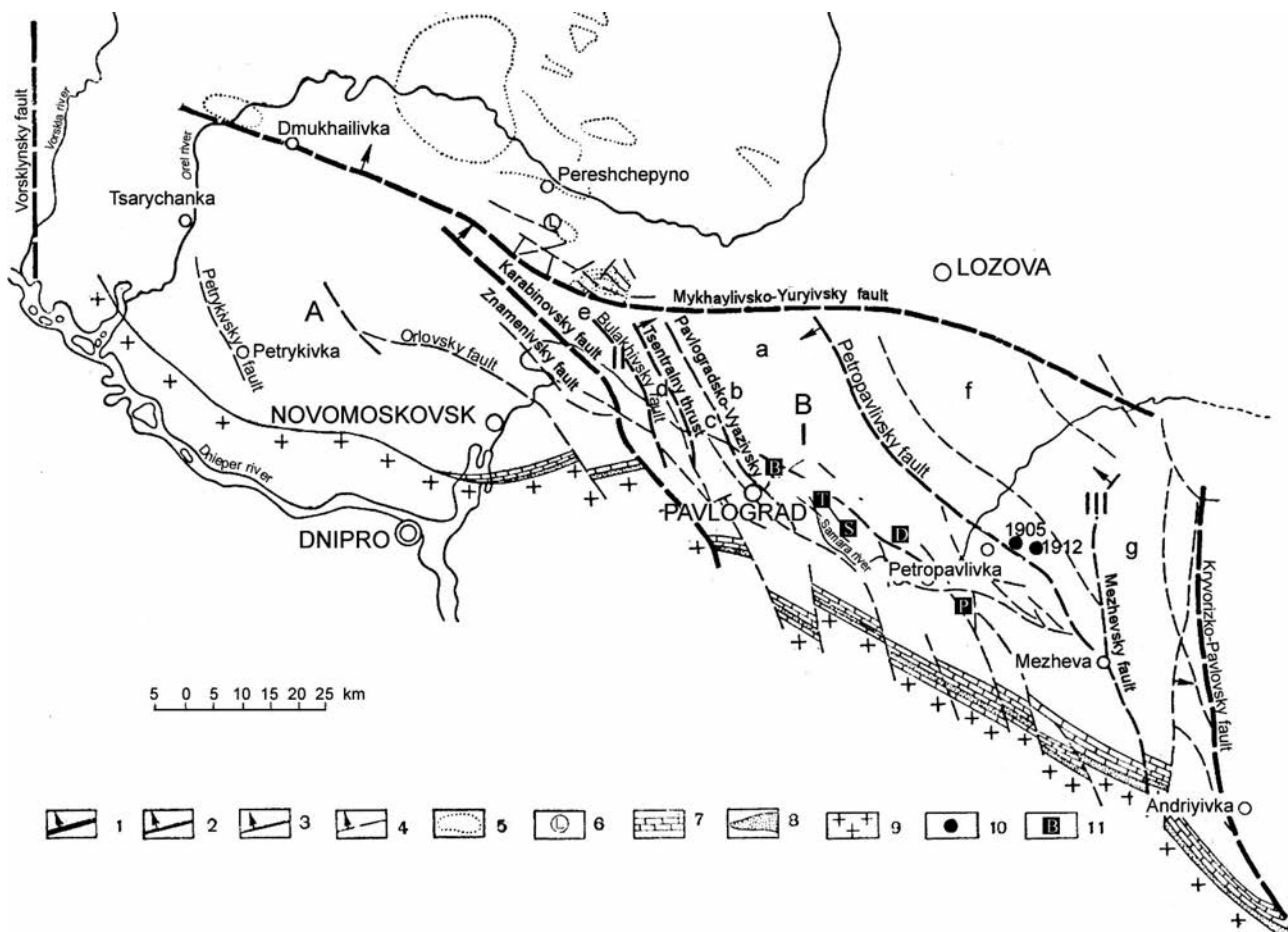
Fig. 2. Tectonic scheme of the Western Donbas [Закономерности..., 1963] with the points of sampling of coal samples Units of the first order: A – Prydniprovsky, B – Samarsky. Blocks of the second order: I – Central; II – Western; III – Eastern. Blocks of the third order: a – Seredniy, b – Samarsky, c – Pavlogradsky, d – Bulakhivsky, e – Karabinovsky, f – Petropavlivsky, g – Mezhevsky. 1 – Fault of the first order; 2 – second order; 3 – third order; 4 – fourth order; 5 – domes; 6 – salt domes; 7 – limestone; 8 – Devonian; 9 – Precambrian; 10 – wells for calculating the erosion of Upper Paleozoic sediments; 11 – mines for which samples of coals for petrology study and for determination of their salinity have been selected: B – Blagodatna, T – Ternovska, S – Samarska, D – Dniprovka, P – Pershotravneva
