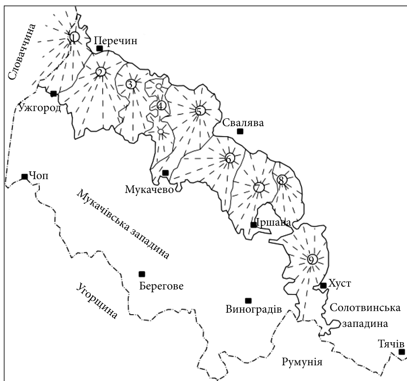
Fig. 1. Scheme of the location of volcanoes of the central type of Vygort-Gutin ridge. Volcanoes: 1 — Poprychny, 2 — Antalivsky, 3 — Makovytsya, 4 — Trostjanytsya (“Three-headed volcano”), 5 — Synyak, 6 — Dehmanov, 7 — Martynsky Kamin, 8 — Buzhora, 9 — Tovsty Verh
